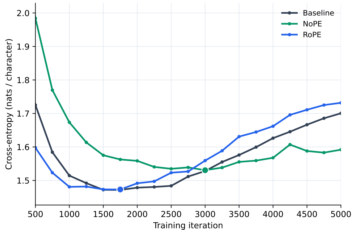
Validation loss (from iteration 500)
