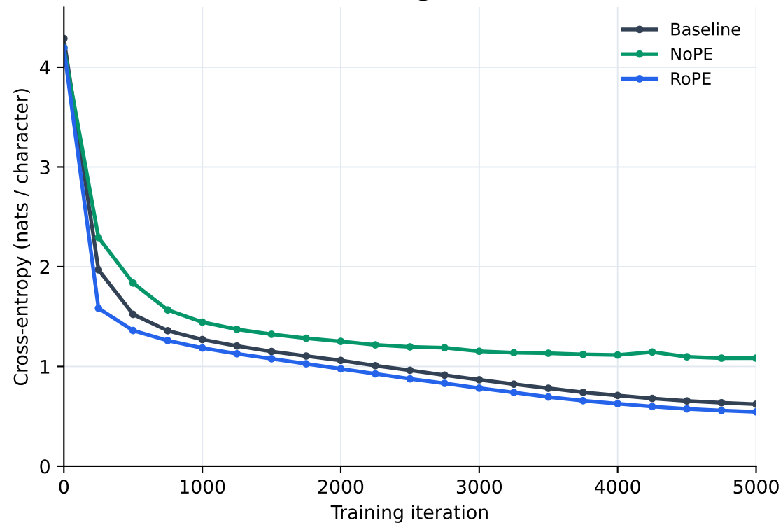
Positions: learned vs. NoPE vs. RoPE Training loss
